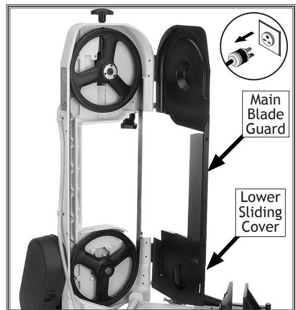
Figure 47. Bandsaw blade guard and the lower sliding cover.
